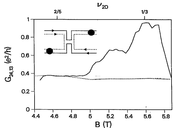
FIG. 5. The excess peak conductance (solid line) and the conductance at V_g=0 (dotted line) as a function of magnetic field for T=45 mK. As the magnetic field varies over the \frac{1}{3} plateau of the unconstricted 2DES, plateaus in the peak conductance are observed near 1(e^2/h) , \frac{2}{3}(e^2/h) , and \frac{1}{3}(e^2/h) . Inset: Depiction of possible mechanism for producing the observed excess conductance peak (see text).
