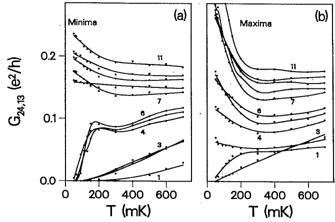
FIG. 3. Conductance of selected (a) minima and (b) maxima from Fig. 2(b) as a function of temperature. Increasing index indicates decreasing V_g or increasing filling factor \nu_c in the constriction. Three different types of temperature dependencies may be distinguished (see text).
