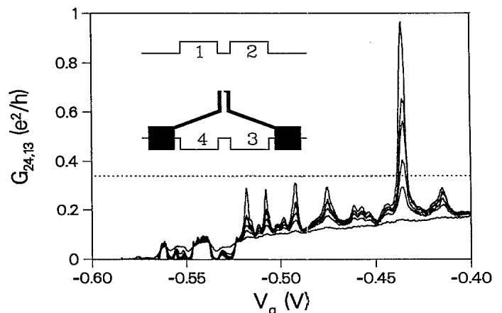
FIG. 1. Conductance as a function of gate voltage for six different temperatures (45, 70, 80, 95, 120, and 200 mK, from top to bottom) at B = 5.7 \text{ T} ( \nu_{2D} = \frac{1}{3} ). The dotted line shows the conductance with V_g = 0 , and is \approx \frac{1}{3}(e^2/h) . The conductance of one peak approaches e^2/h , exceeding the bulk conductance. Inset: Schematic drawing of device geometry with the gates shaded and the contacts labeled 1-4. The magnetic field points into the page.
