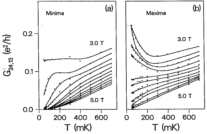
FIG. 4. Conductance of the (a) minimum and (b) maximum labeled 3 in Fig. 2(b), as a function of temperature for eleven equally spaced magnetic fields ranging from B=3.0 ( \nu_{2D}=0.62 ) to 5.0 T ( \nu_{2D}=0.37 ). Note the similarity to Fig. 3.
