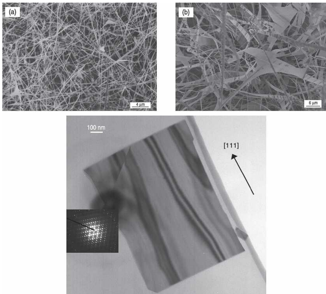
Fig. 1. SEM images of \beta\text{-Ga}_2\text{O}_3 (a) nanowires and (b) nanobelts synthesized at 950^{\circ}\text{C} and 1,050^{\circ}\text{C} , respectively. (c) HRTEM image of a single \beta\text{-Ga}_2\text{O}_3 nanobelt along the [111] growth direction. Inset is a SAD pattern revealing the monoclinic structure.
