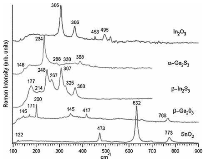
Fig. 3. Micro-Raman spectra from semiconducting nanowires.
