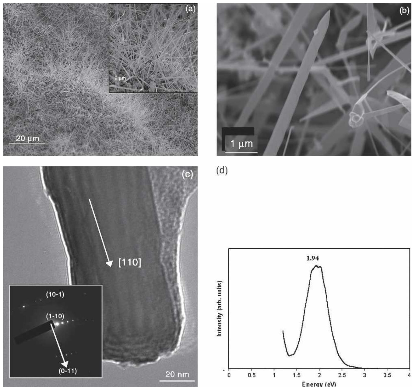
Fig. 4. (a) SEM figure of SnO_2 nanowires prepared at 900^\circ C . The inset is a blown up image of the nanowires. (b) SEM image of SnO_2 nanobelts prepared at 1,200^\circ C . (c) HRTEM image of a single SnO_2 nanowire and the corresponding diffraction pattern. (d) Photoluminescence spectrum of SnO_2 nanowires.
