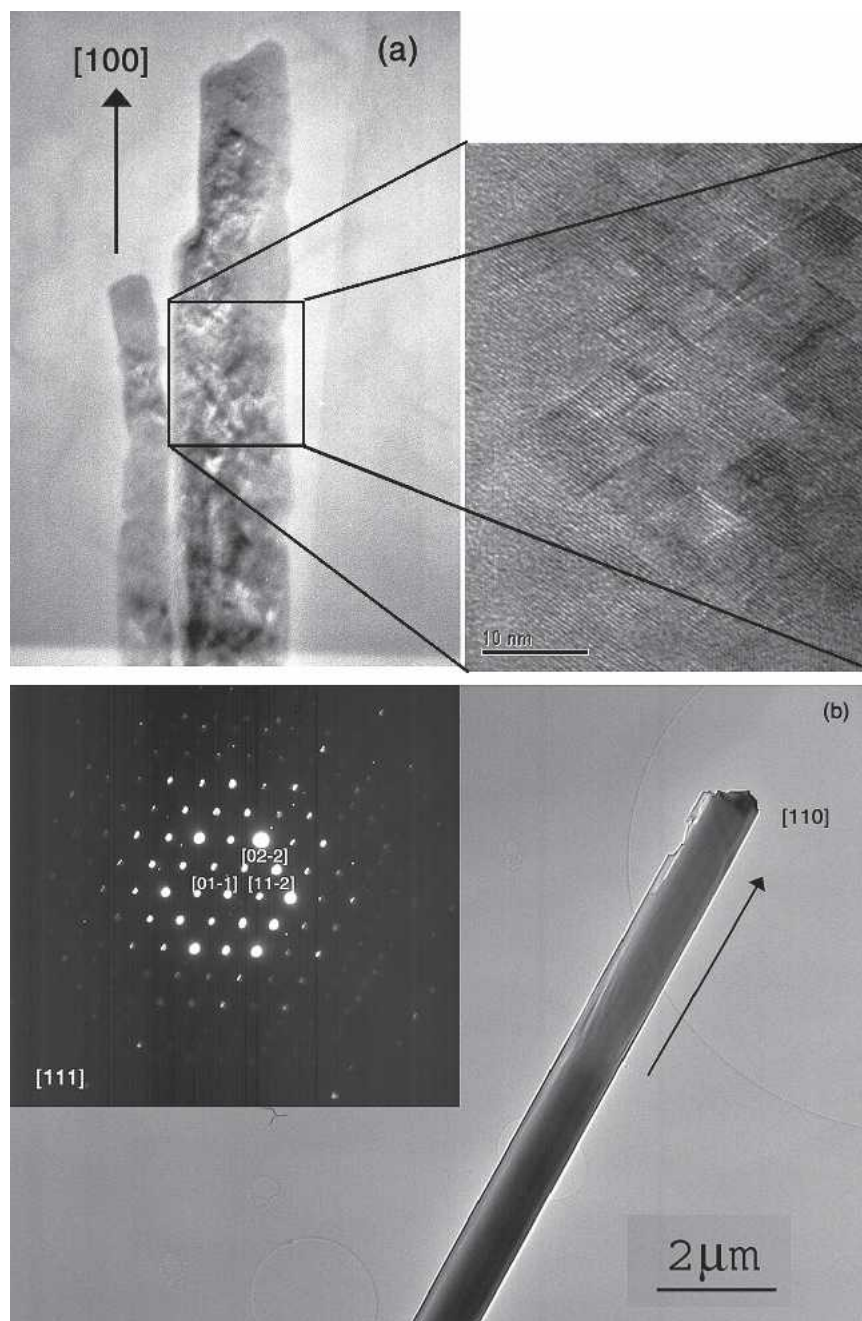
Fig. 2. (a) HRTEM image of a \alpha - \text{Ga}_2\text{S}_3 nanowire showing twinning shown in detail in the inset figure. (b) HRTEM image of a \beta - \text{In}_2\text{S}_3 nanowire exhibiting tetragonal crystal structure (inset figure shows the SAD pattern).
